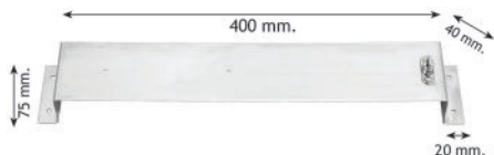
Bracket for folding panels with fixing bolt.
