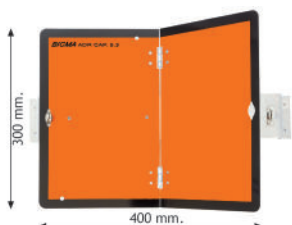
A.D.R. vertical folding panel with bracket. Al: Aluminium
