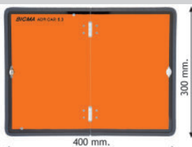
Aluminium, stainless steel and zinc plated A.D.R. vertical folding panel with rubber protection, clip in the centre. Al: Aluminium Aisi: Stainless steel Fe-Zn: Zinc plated
